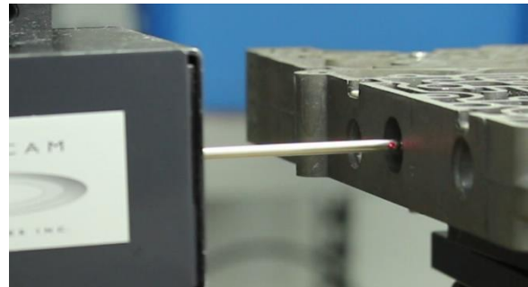
Figure 1: The rotating optical probe of the BOREINSPECT system scans a valve-body bore ID as it moves into the bore
