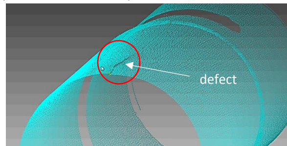
Figure 2: The acquired 3D map of a bore ID in the above valve body reveals a defect next to the bore opening.
