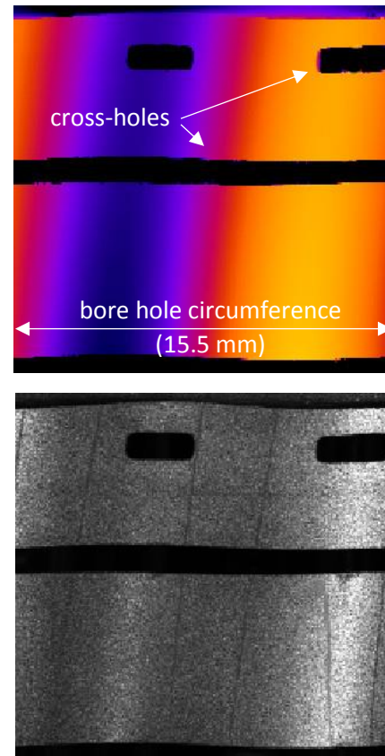
Figure 4 Height image (top) and intensity image (bottom) of the unfolded bore interior.
