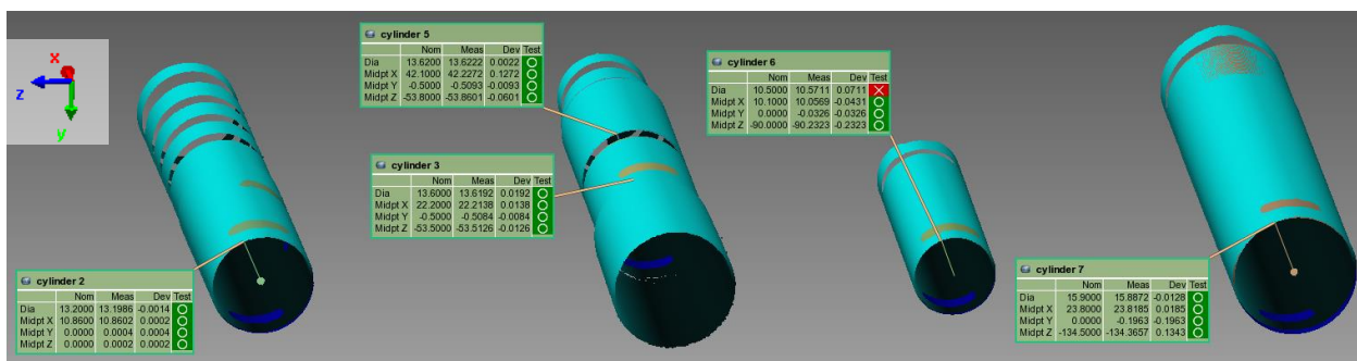
Figure 5: Four bores in a valve body were scanned and analyzed in one inspection sequence. The results include dimensional measurements and pass/fail reporting for each bore, as well as the bore pitch (bore spacing), and exact positioning of each bore on the valve body.
