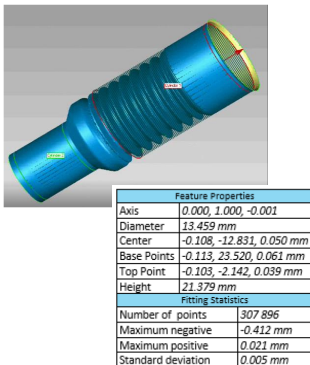
Figure 6: 3D map and thread measurements for the inner thread of a turbocharger impeller. The high-precision measurements were calculated from 307,000 3D points acquired in ~4 seconds.
