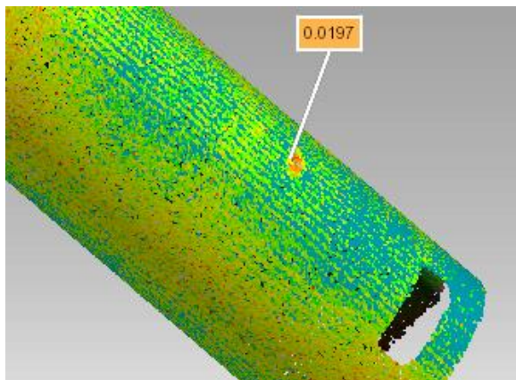
Figure 3: Deviation map (viewed with PolyWorks Inspector™) highlights a bore ID surface defect – a 19.7 µm deep pit.
